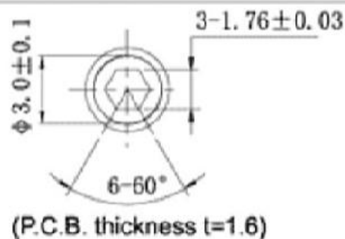
Shaft hole shape and dimension
